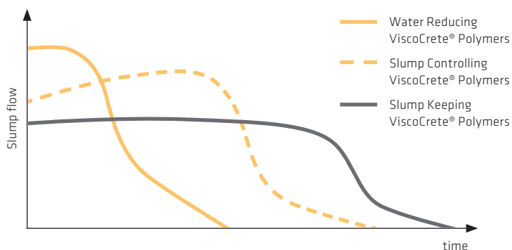
Examples for consistency curves of various PCEs
