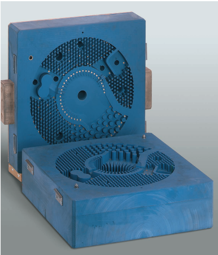
High durability with SikaBlock® M980 for foundry core boxes even in complicated shapes
