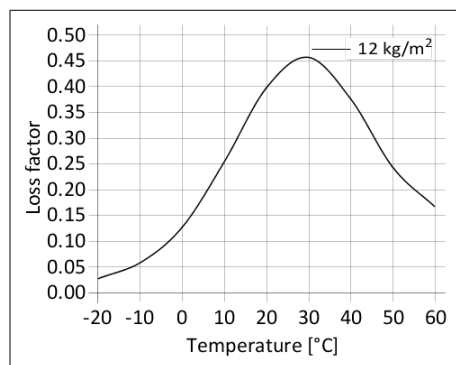
Diagram 1: Loss factor SikaDamp®-140 V at 200 Hz
