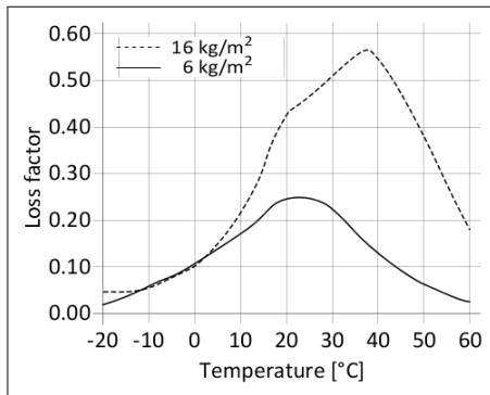
Diagram 1: Loss factor SikaDamp®-146 at 200 Hz
