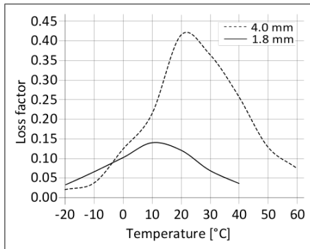
Diagram 1: Loss factor SikaDamp®-111 at 200 Hz
