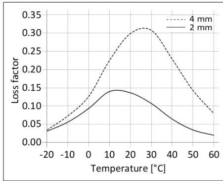
Diagram 1: Loss factor SikaDamp®-112 at 200 Hz
