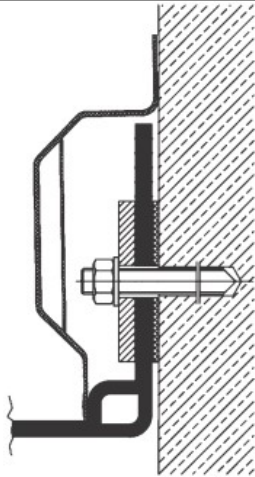
Example of a loose/fixed flange joint design
