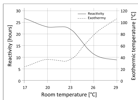
Diagram 1: casted in plastic cup – 630 g, Ø 85 mm, height 90 mm
