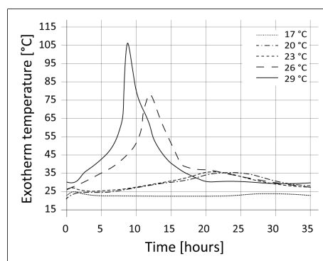
Diagram 2: casted in plastic cup – 630 g, Ø 85 mm, height 90 mm
