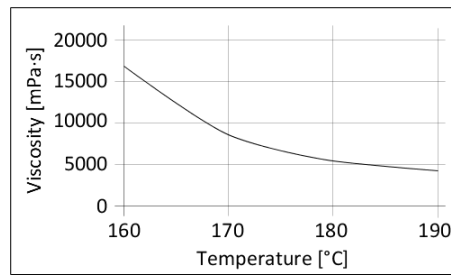
Diagram 1: Viscosity as a function of temperature SikaMelt®-285 FR
