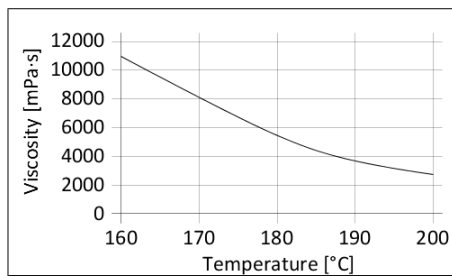
Diagram 1: Viscosity of SikaMelt®-174 as function of temperature
