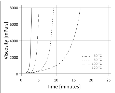
Diagram 1: Viscosity development
