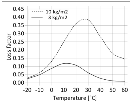
Diagram 1: Loss factor SikaDamp®-140 PES at 200 Hz
