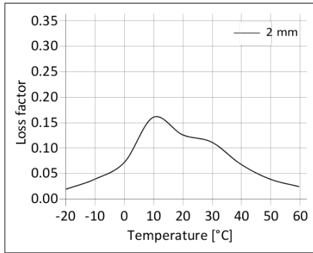
Diagram 1: loss factor SikaDamp®-110 PP at 200 Hz
