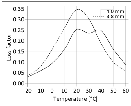
Diagram 1: Loss factor SikaDamp®-113 at 200 Hz
