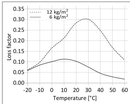
Diagram 1: Loss factor SikaDamp®-144 at 200 Hz
